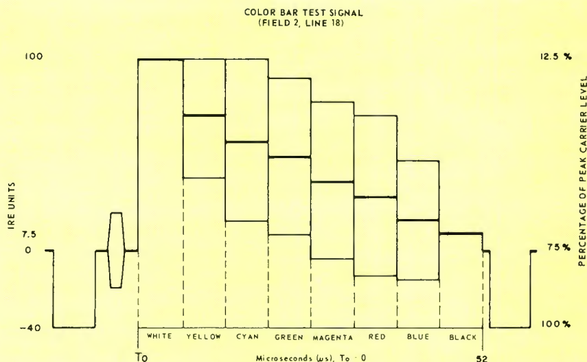
Fig. 2 VIT waveform required for field 2, line 18.
