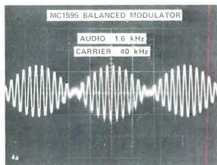
Fig. 4a Scope pattern for the MC1595 balanced modulator.
