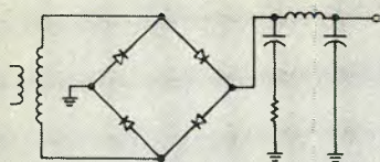
SINGLE PHASE FULL WAVE BRIDGE PRV 141.4% OF DC OUT PER RECTIFIER CURRENT 50% OF DC1 PER RECTIFIER
