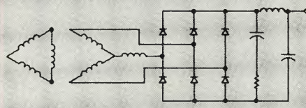
3 PHASE FULL WAVE BRIDGE PRV PER RECTIFIER 105% OF DC PER RECTIFIER CURRENT 33.3% OF DC1 PER RECTIFIER
