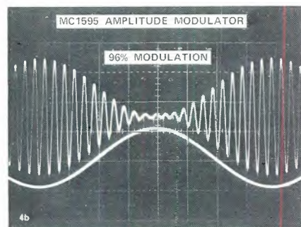
Fig. 4b Scope pattern for the MC1595 as a modulator.
