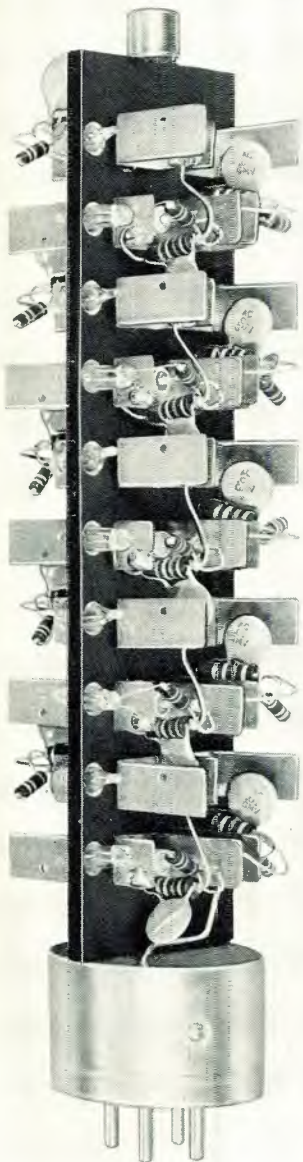
Fig. 1. This 20 kV, 6 Ampere stack replaces the 673.
