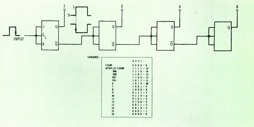
Fig. 3 Down-counter (binary).
