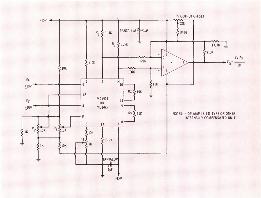
Fig. 7. Direct coupled general purpose multiplier with buffered output.
